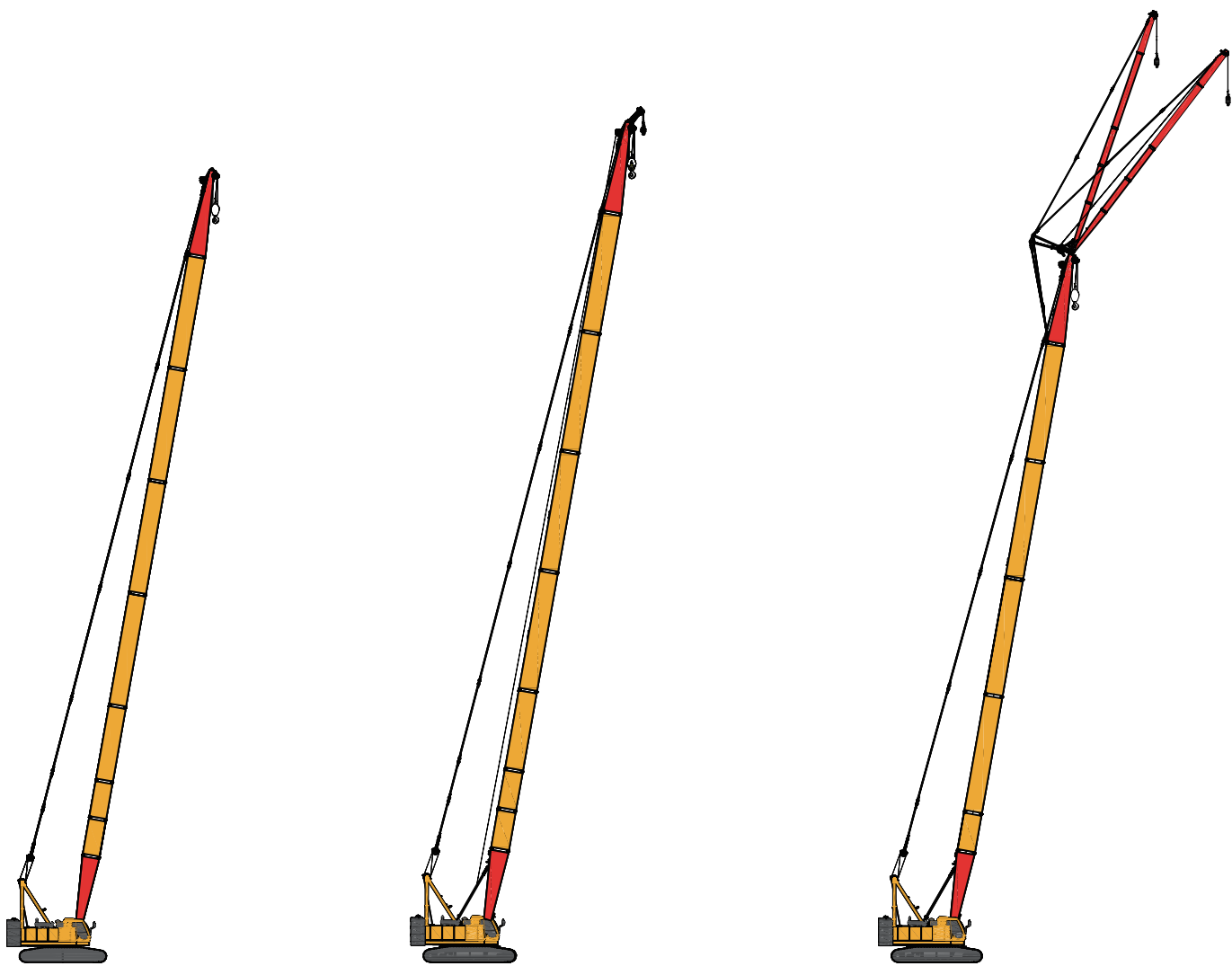
Main boom operation mode HB
