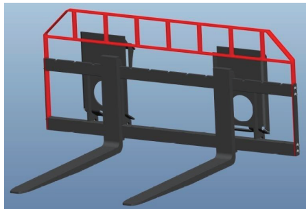
Fork - Technical Data
